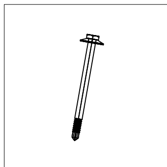
Tornillo Taladro 5.5*112 (panel 82 mm) REF: 85285
