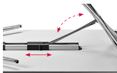
Sliding movement detail
